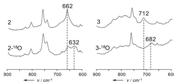
Figure 2. Top: UV/Vis spectra for the titration process from 2 to 3 (1 mm). Bottom: Raman spectra of complexes 2 and 3 in CH 3 CN, and the corresponding complexes after addition of H 2 18 O ( 2 - 18 O and 3 - 18 O).
